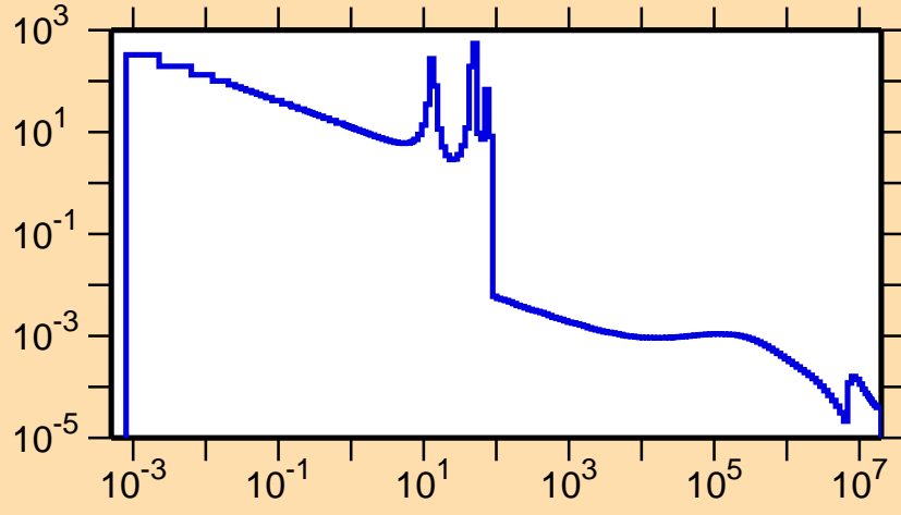
\sigma vs. E for ^{91}\text{Rh}(n,\gamma)
