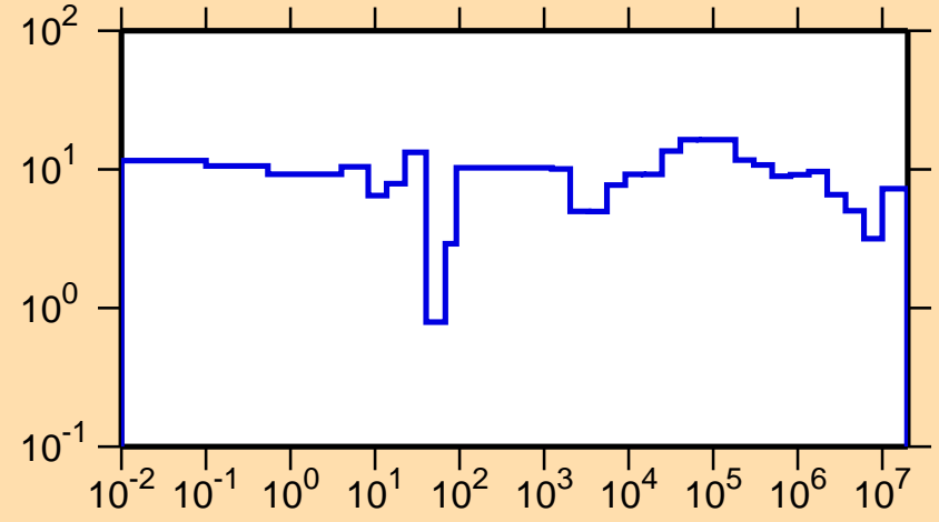
\Delta\sigma/\sigma vs. E for ^{91}\text{Rh}(n,\text{tot.})
