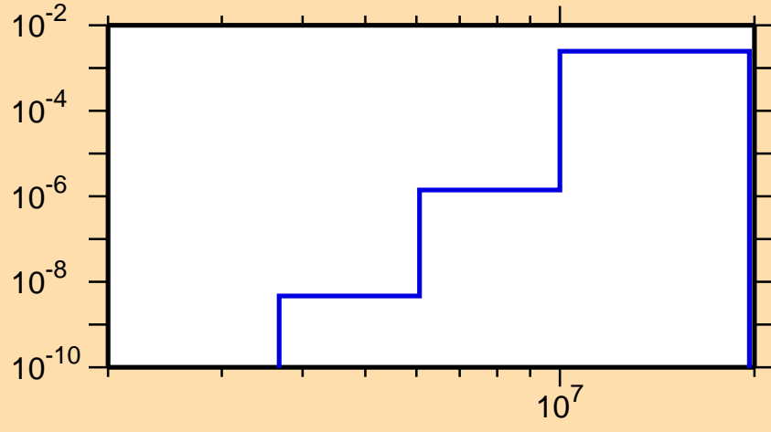
\sigma vs. E for ^{91}\text{Rh}(n,\text{He}3)
