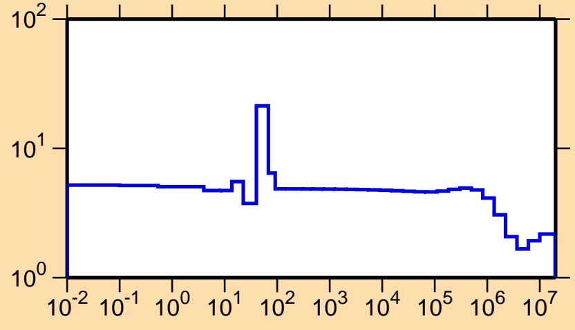
\sigma vs. E for ^{91}\text{Rh}(n,\text{el.})
