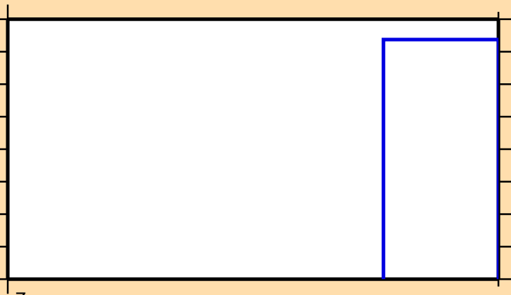
\sigma vs. E for ^{92}\text{Rh}(n,nt)
