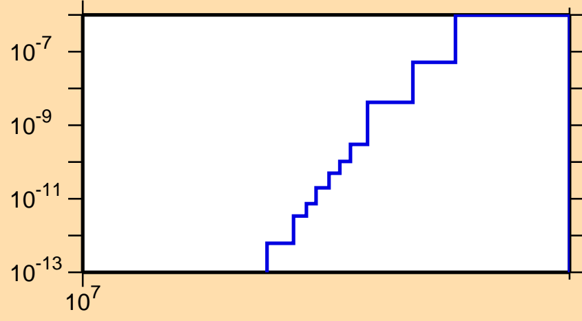
\sigma vs. E for ^{92}\text{Rh}(\text{mt } 45)
