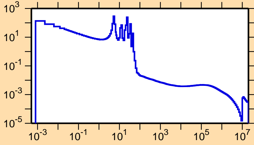
\sigma vs. E for ^{92}\text{Rh}(n,\gamma)
