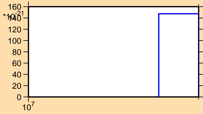
\sigma vs. E for ^{92}\text{Rh}(n,nt)
