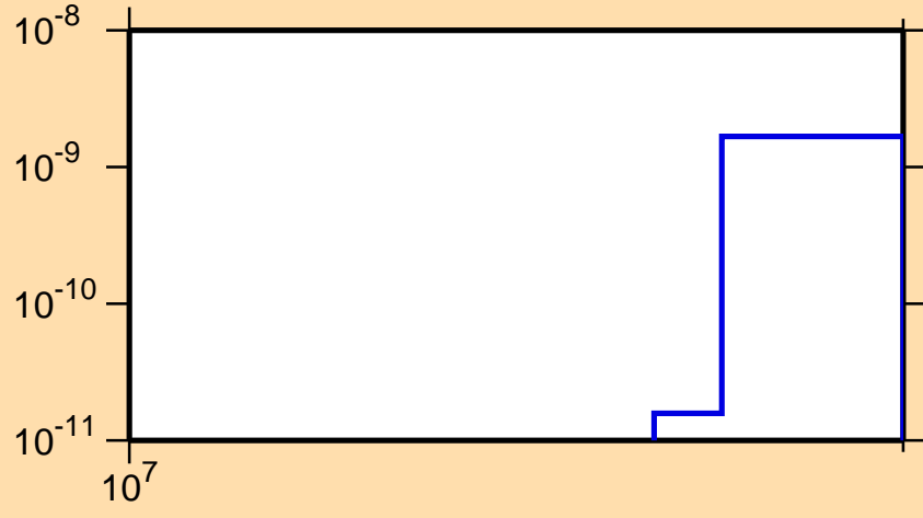
\sigma vs. E for ^{92}\text{Rh}(\text{mt } 34)
