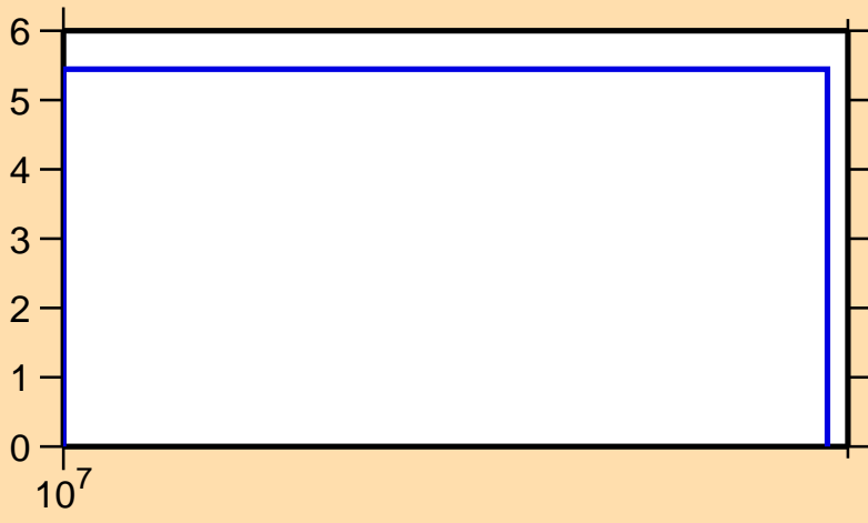
\Delta\sigma/\sigma vs. E for ^{92}\text{Rh}(n,\text{el.})
