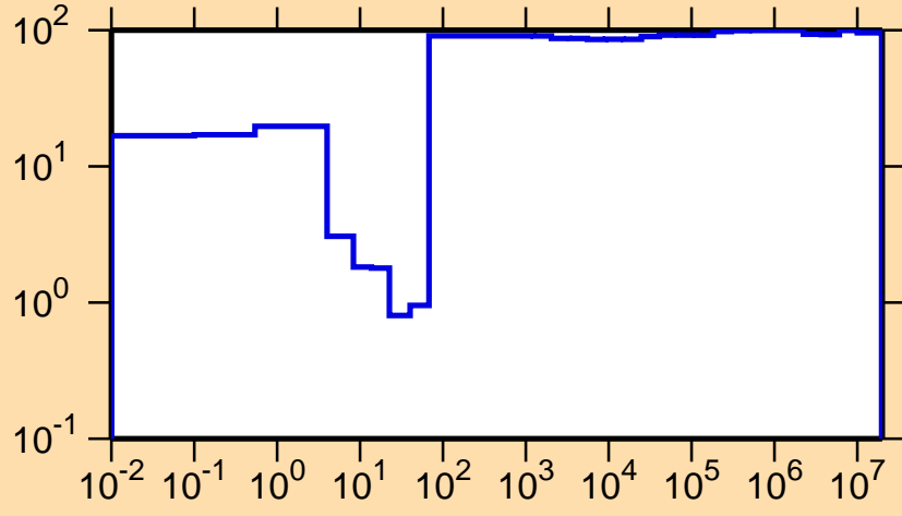
\Delta\sigma/\sigma vs. E for ^{92}\text{Rh}(n,\gamma)
