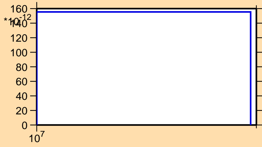
\sigma vs. E for ^{92}\text{Rh}(\text{mt117})
