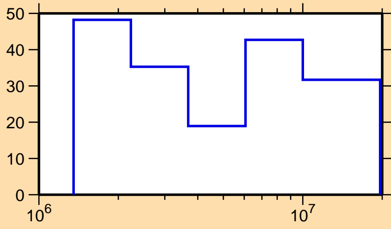
\Delta\sigma/\sigma vs. E for ^{92}\text{Rh}(n,n_1)
