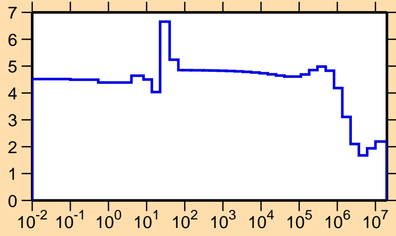
\sigma vs. E for ^{92}\text{Rh}(n,\text{el.})
