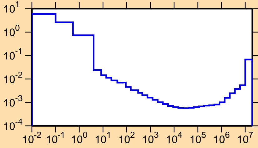
\sigma vs. E for ^{92}\text{Rh}(n,\alpha)
