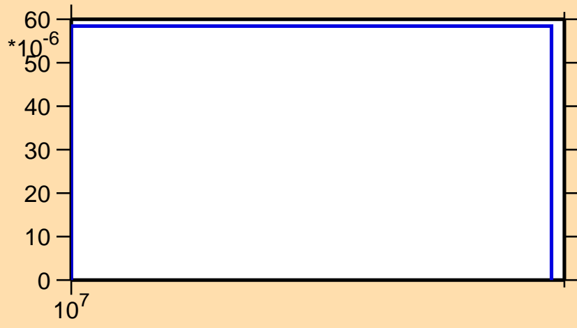
\sigma vs. E for ^{92}\text{Rh}(n,2n)
