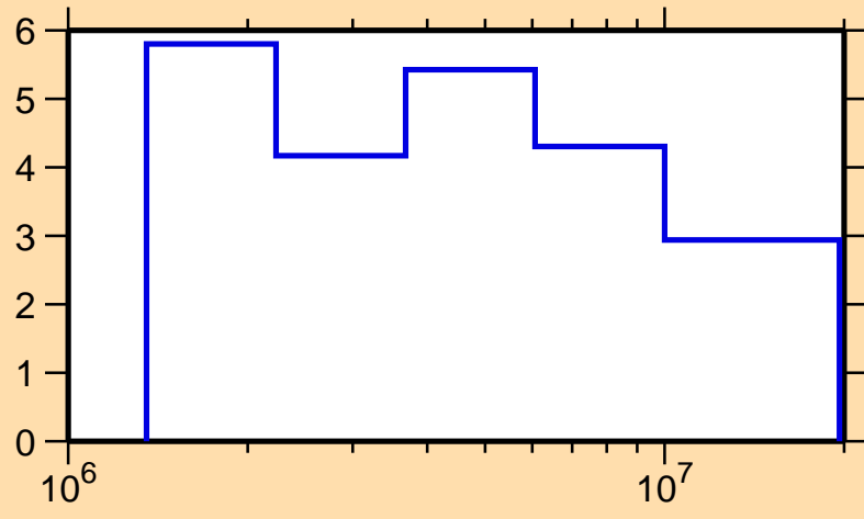
\Delta\sigma/\sigma vs. E for ^{92}\text{Rh}(n,\text{tot.})
