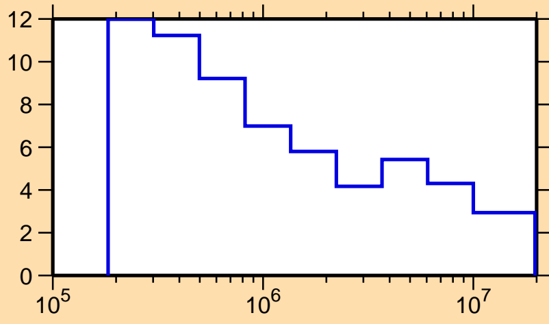
\Delta\sigma/\sigma vs. E for ^{92}\text{Rh}(n,\text{tot.})
