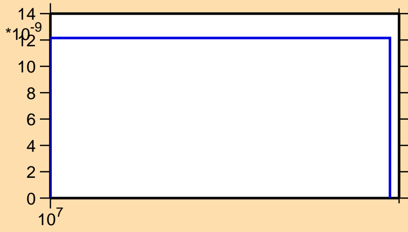
\sigma vs. E for ^{92}\text{Rh}(\text{mt } 45)
