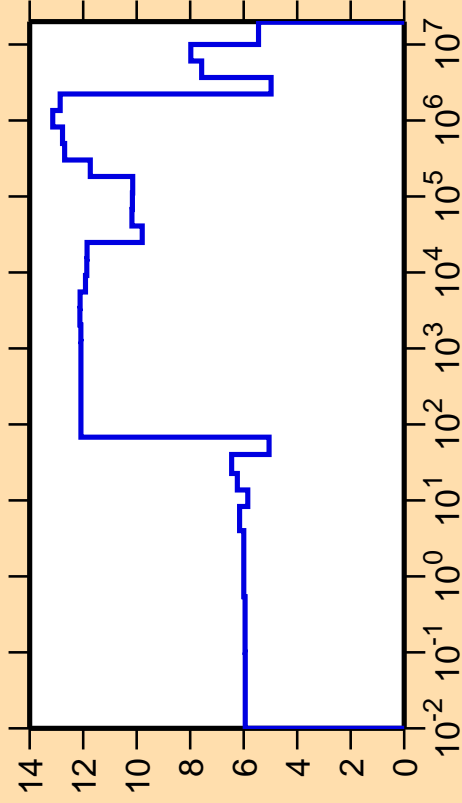
\Delta\sigma/\sigma vs. E for ^{92}\text{Rh}(n,\text{el.})
