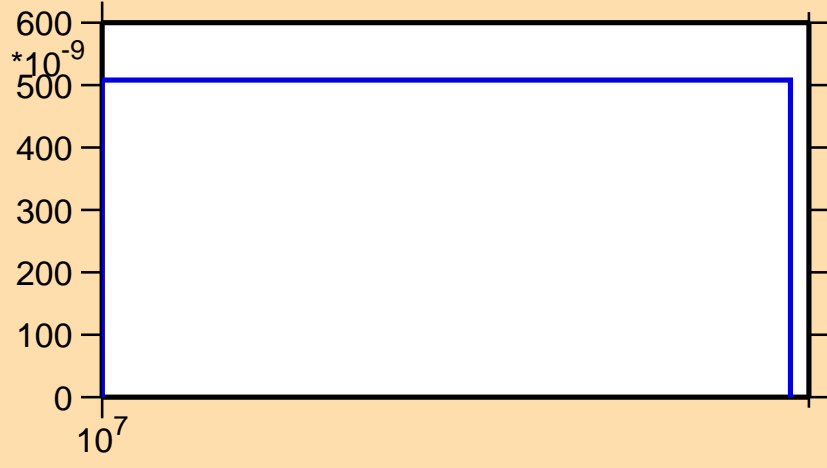
\sigma vs. E for ^{92}\text{Rh}(n,\text{pt})
