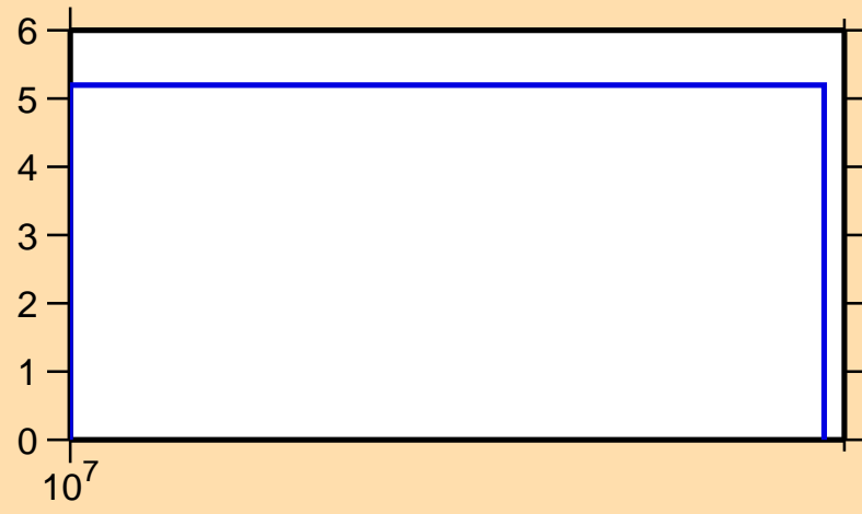
\Delta\sigma/\sigma vs. E for ^{92}\text{Rh}(n,\text{nonel.})
