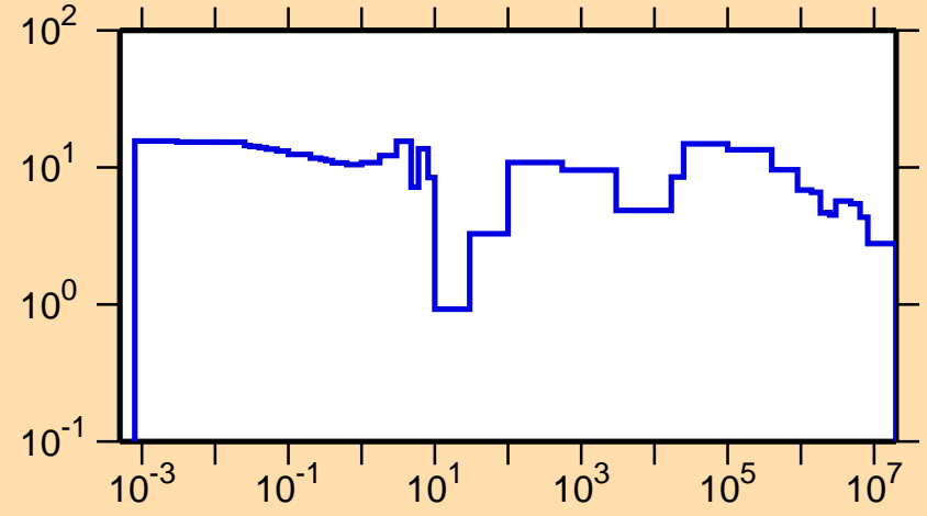
\Delta\sigma/\sigma vs. E for ^{92}\text{Rh}(n,\text{tot.})
