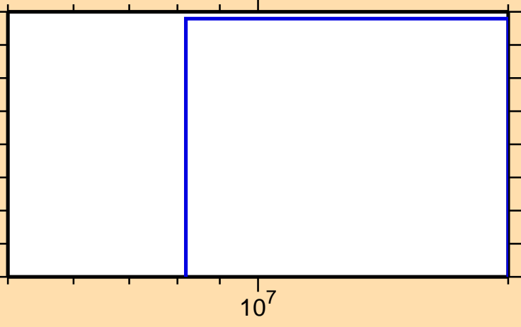
\sigma vs. E for ^{92}\text{Rh}(n,n\alpha)
