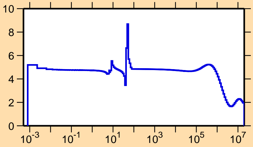
\sigma vs. E for ^{93}\text{Rh}(n,\text{el.})
