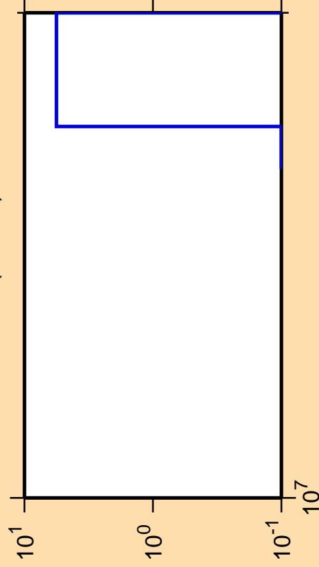
\Delta\sigma/\sigma vs. E for ^{93}\text{Rh} (mt 34)
