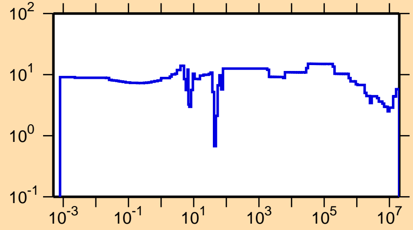
\Delta\sigma/\sigma vs. E for ^{93}\text{Rh}(n,\text{tot.})
