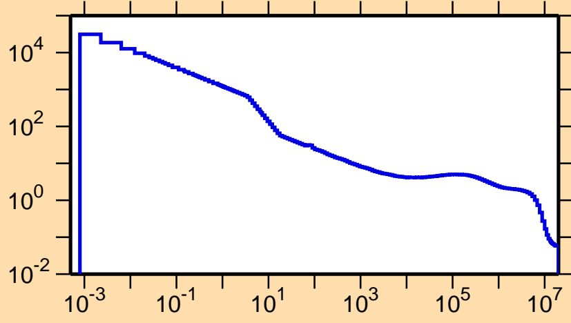
\sigma vs. E for ^{93}\text{Rh}(n,p)
