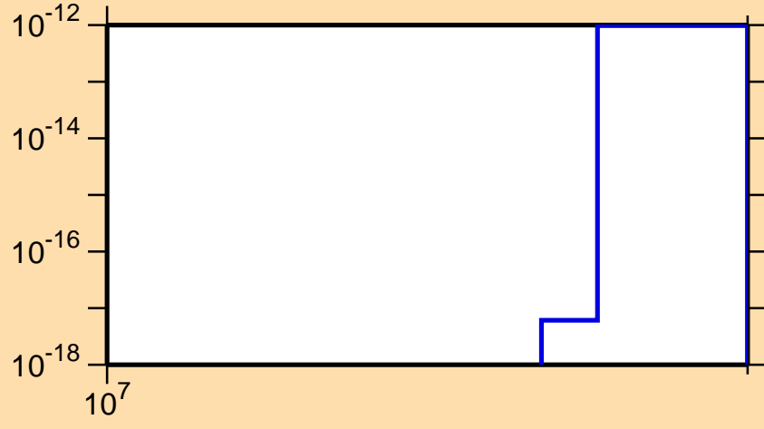
\sigma vs. E for ^{93}\text{Rh} (mt 34)
