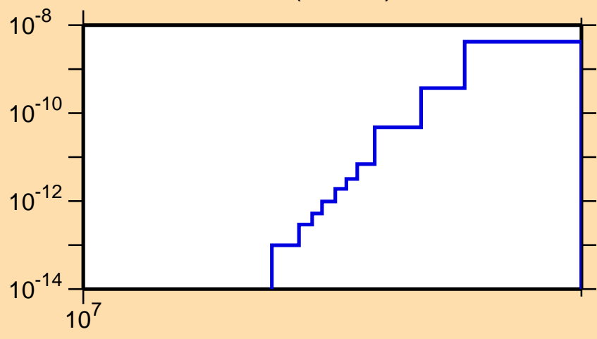
\sigma vs. E for ^{93}\text{Rh}(\text{mt117})
