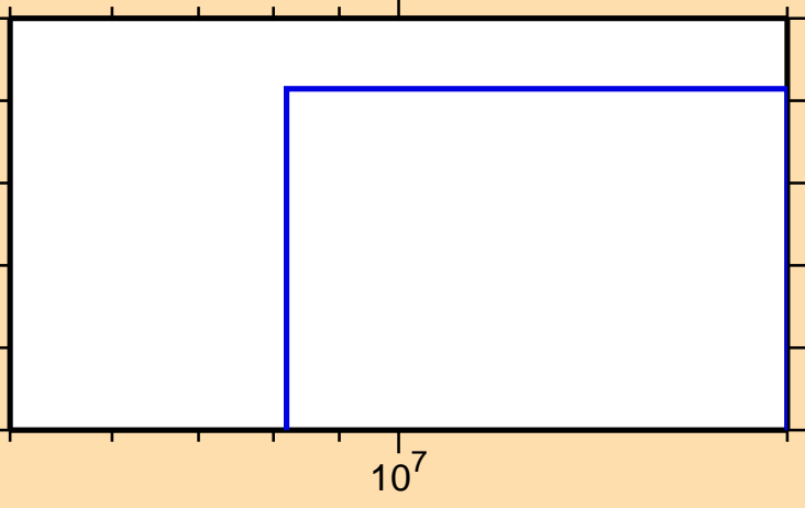
\sigma vs. E for ^{93}\text{Rh}(n,2np)
