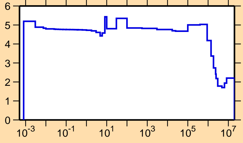
\sigma vs. E for ^{93}\text{Rh}(n,\text{el.})
