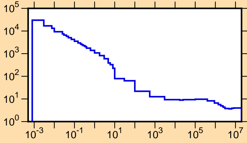
\sigma vs. E for ^{93}\text{Rh}(n,\text{tot.})
