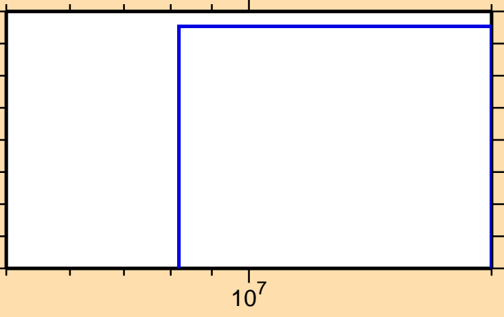
\sigma vs. E for ^{93}\text{Rh}(n,\text{pd})
