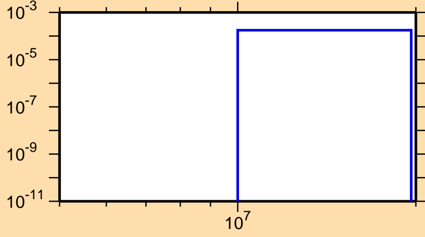
\sigma vs. E for ^{94}\text{Rh}(n,pd)
