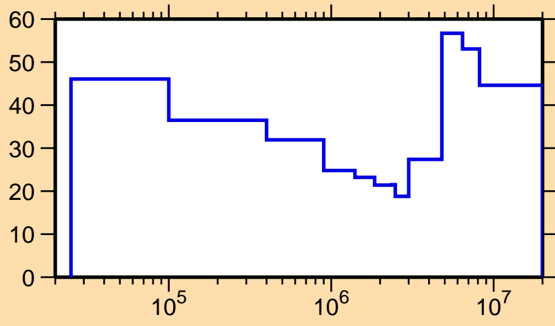
\Delta\sigma/\sigma vs. E for ^{94}\text{Rh}(n,n_1)
