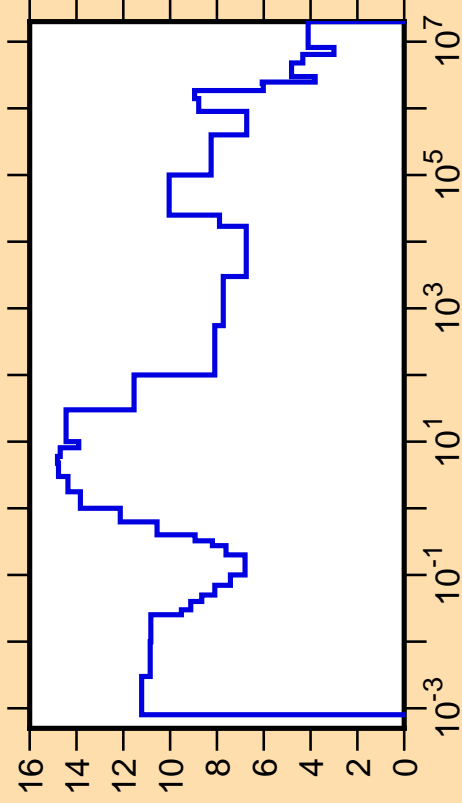
\Delta\sigma/\sigma vs. E for ^{94}\text{Rh}(n,\text{tot.})
