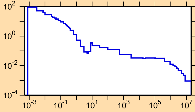
\sigma vs. E for ^{94}\text{Rh}(n,\gamma)
