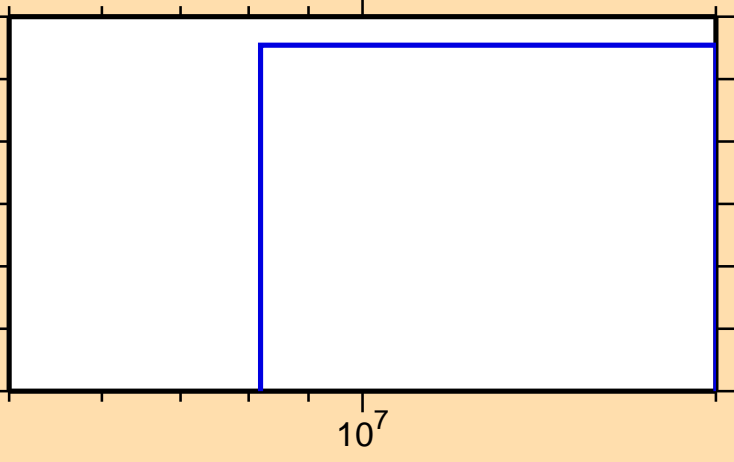
\sigma vs. E for ^{94}\text{Rh}(n,\text{pt})
