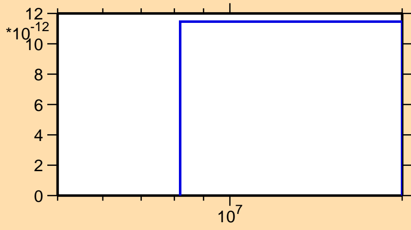
\sigma vs. E for ^{94}\text{Rh}(\text{mt117})
