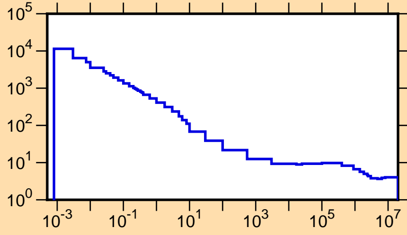
\sigma vs. E for ^{94}\text{Rh}(n,\text{tot.})
