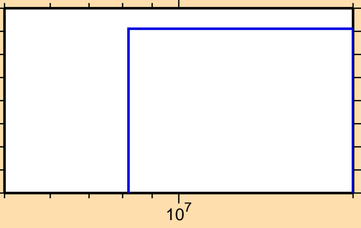
\sigma vs. E for ^{94}\text{Rh}(n,\text{pd})
