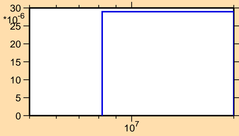
\sigma vs. E for ^{94}\text{Rh}(n,n\alpha)
