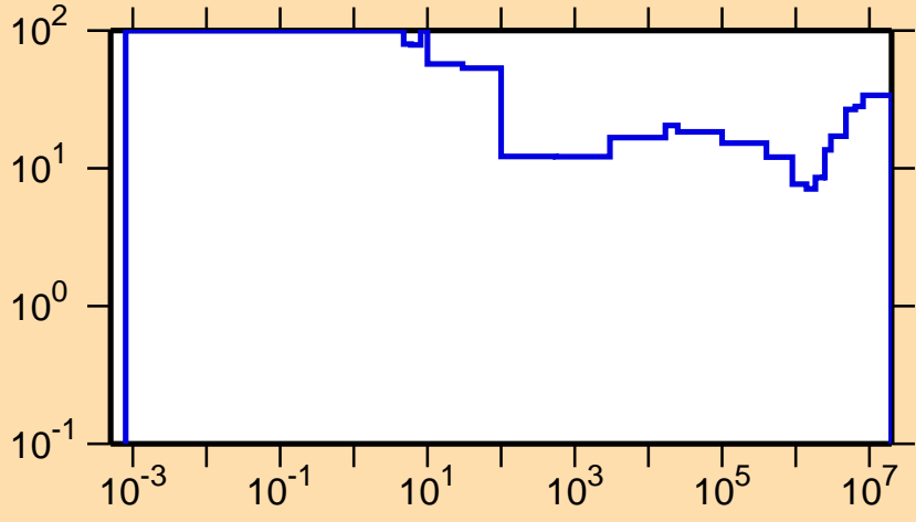
\Delta\sigma/\sigma vs. E for ^{94}\text{Rh}(n,p)
