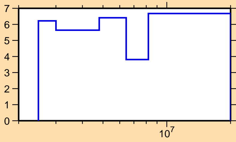
\Delta\sigma/\sigma vs. E for ^{94}\text{Rh}(n,\text{el.})
