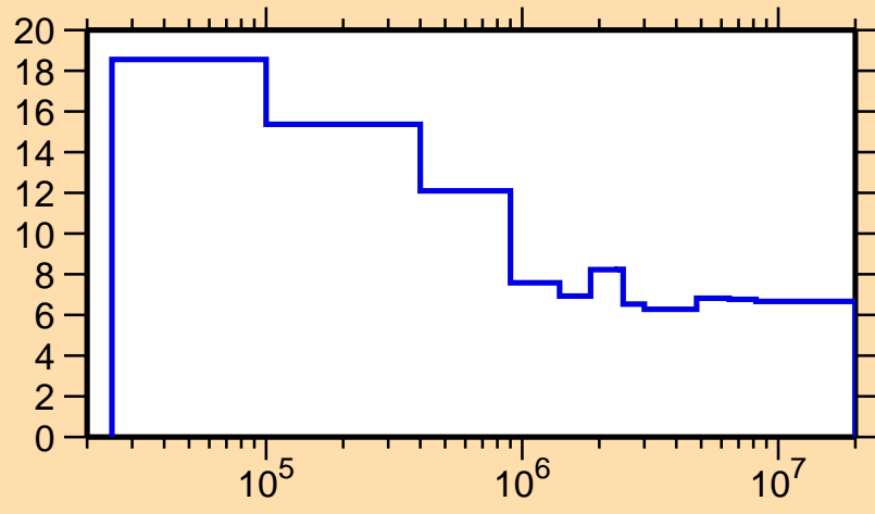
\Delta\sigma/\sigma vs. E for ^{94}\text{Rh}(n,\text{nonel.})
