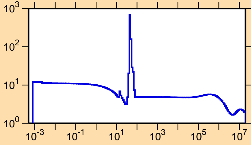
\sigma vs. E for ^{94}\text{Rh}(n,\text{el.})
