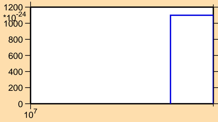
\sigma vs. E for ^{94}\text{Rh}(n,nt)
