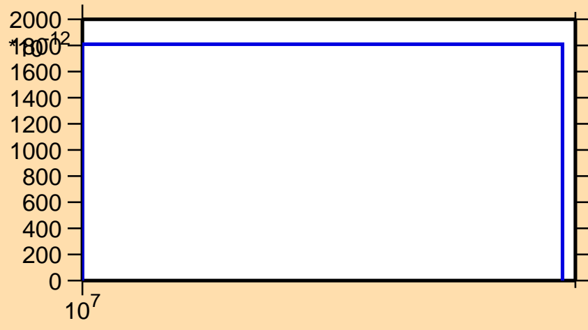
\sigma vs. E for ^{94}\text{Rh}(\text{mt } 45)
