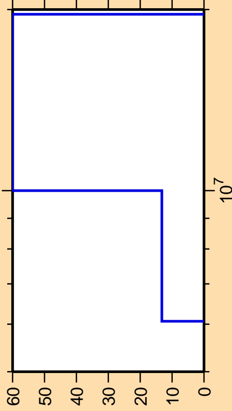
\Delta\sigma/\sigma vs. E for ^{94}\text{Rh}(n,n\alpha)
