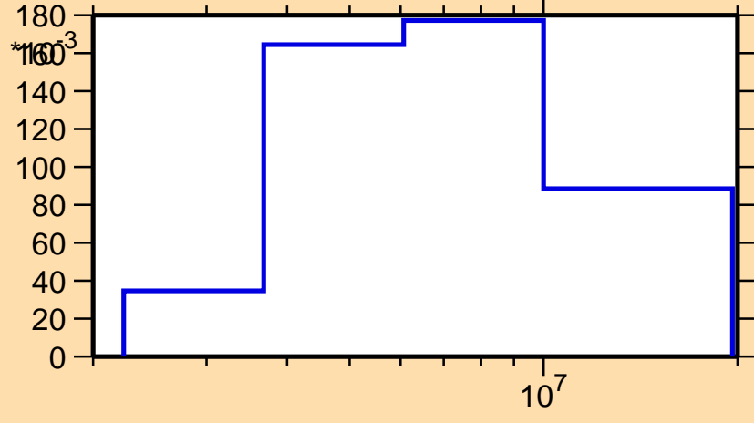
\sigma vs. E for ^{94}\text{Rh}(n,n\text{cont.})
