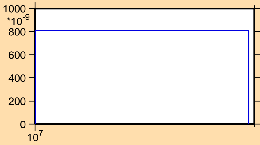
\sigma vs. E for ^{94}\text{Rh}(n,2np)
