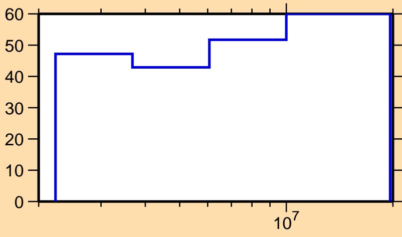
\Delta\sigma/\sigma vs. E for ^{94}\text{Rh}(n,n\text{cont.})
