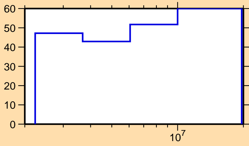
\Delta\sigma/\sigma vs. E for ^{94}\text{Rh}(n,ncont.)
