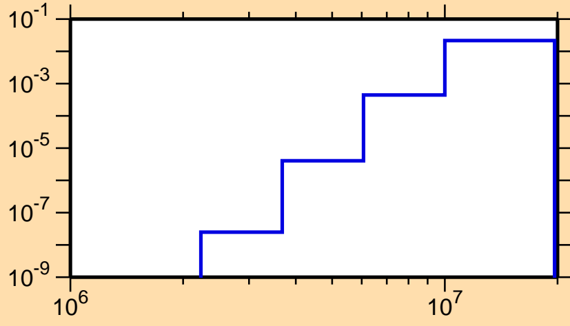
\sigma vs. E for ^{94}\text{Rh}(n,d)
