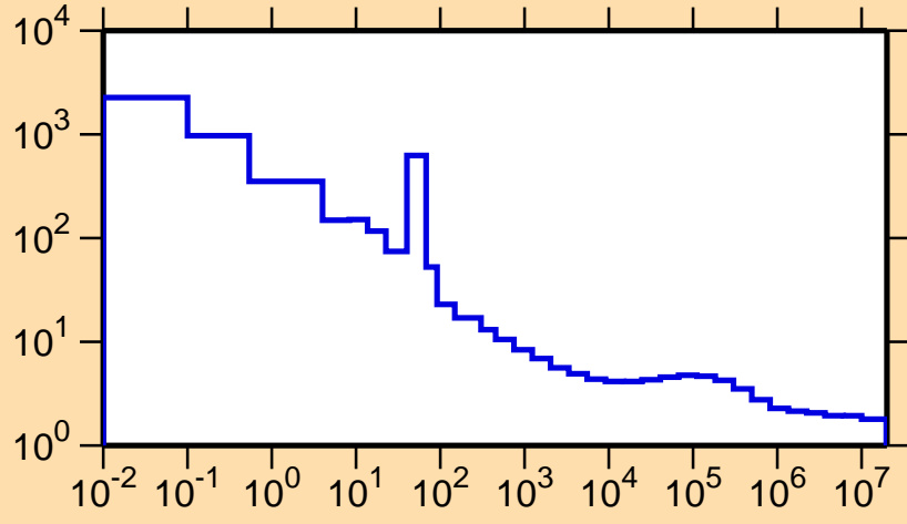
\sigma vs. E for ^{94}\text{Rh}(n,\text{nonel.})
