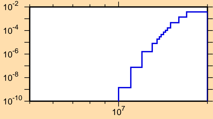
\sigma vs. E for ^{95}\text{Rh}(n,\alpha)
