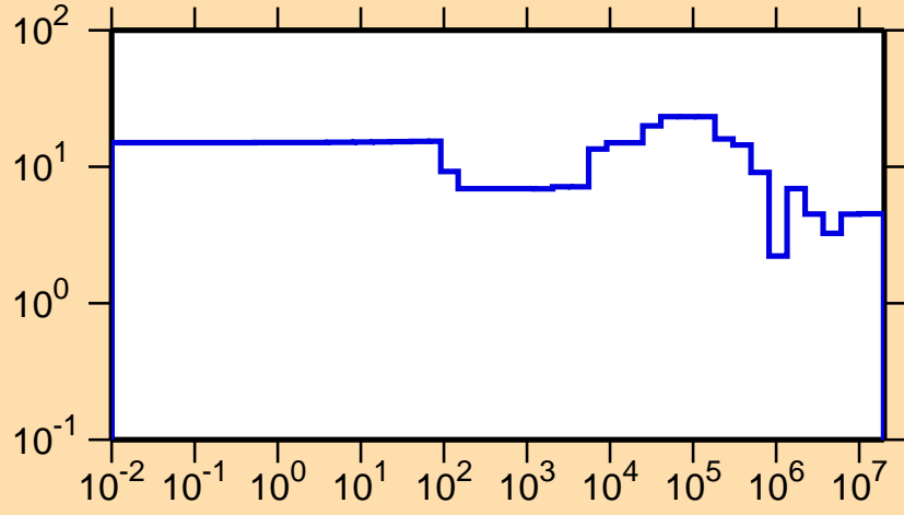
\Delta\sigma/\sigma vs. E for ^{95}\text{Rh}(n,el.)
