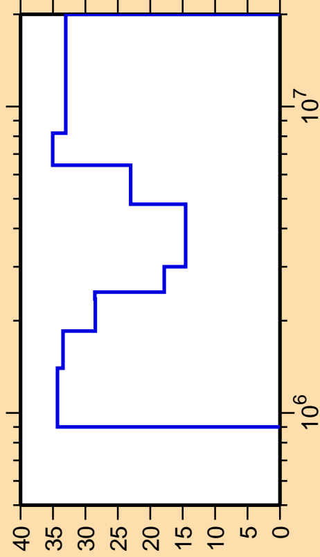
\Delta\sigma/\sigma vs. E for ^{95}\text{Rh}(n,n_3)
