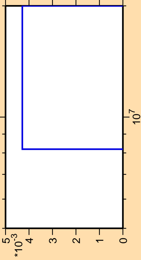
\Delta\sigma/\sigma vs. E for ^{95}\text{Rh}(\text{mt } 34)
