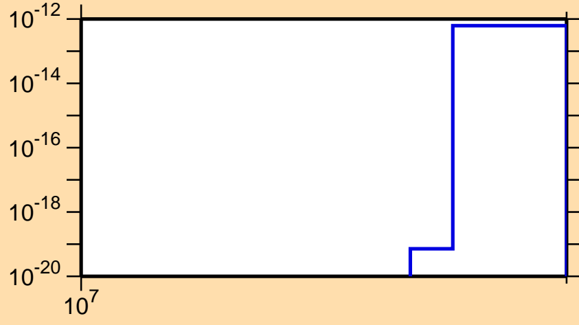
\sigma vs. E for ^{95}\text{Rh} (mt 34)
