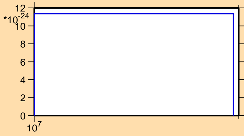
\sigma vs. E for ^{95}\text{Rh}(n,nt)
