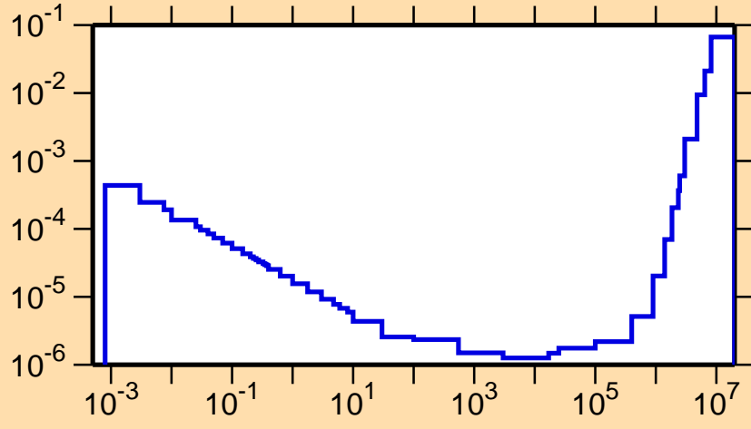
\sigma vs. E for ^{95}\text{Rh}(n,\alpha)
