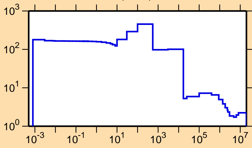
\sigma vs. E for ^{95}\text{Rh}(n,\text{el.})
