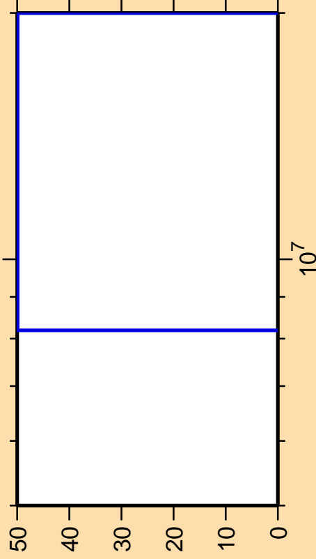
\Delta\sigma/\sigma vs. E for ^{95}\text{Rh}(\text{mt } 45)
