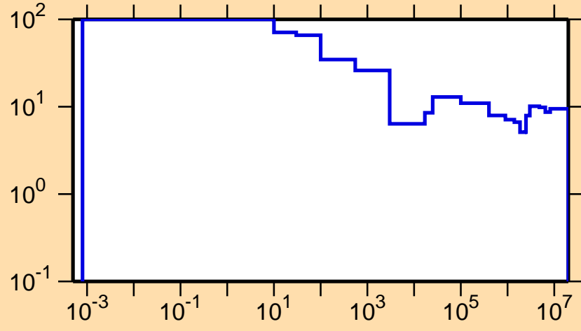
\Delta\sigma/\sigma vs. E for ^{95}\text{Rh}(n,p)
