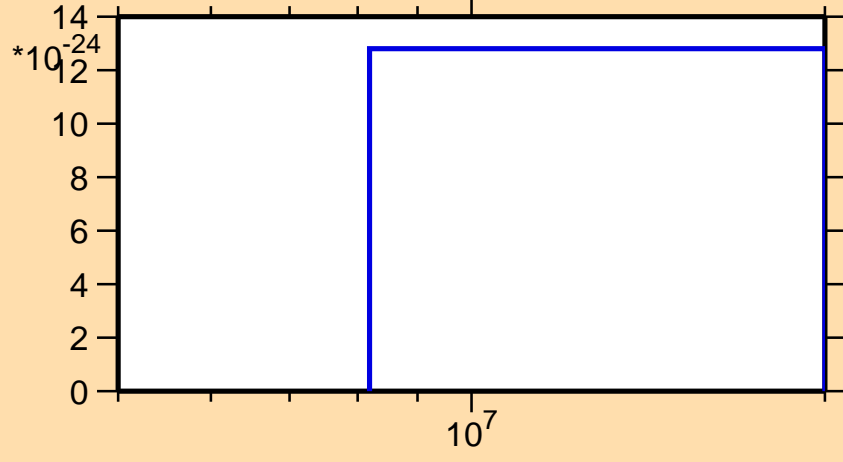
\sigma vs. E for ^{95}\text{Rh}(n,nt)
