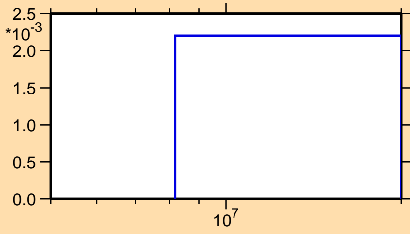
\sigma vs. E for ^{95}\text{Rh}(n,2n)
