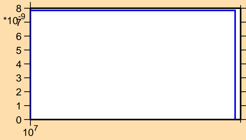
\sigma vs. E for ^{96}\text{Rh} (mt 45)
