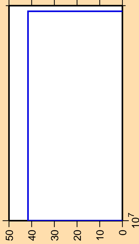
\Delta\sigma/\sigma vs. E for ^{96}\text{Rh} (mt 45)
