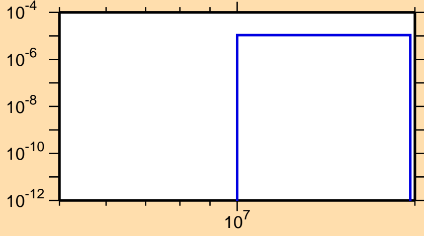
\sigma vs. E for ^{96}\text{Rh}(n,pd)
