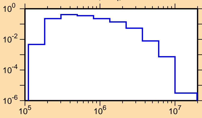
\sigma vs. E for ^{96}\text{Rh}(n,n_4)
