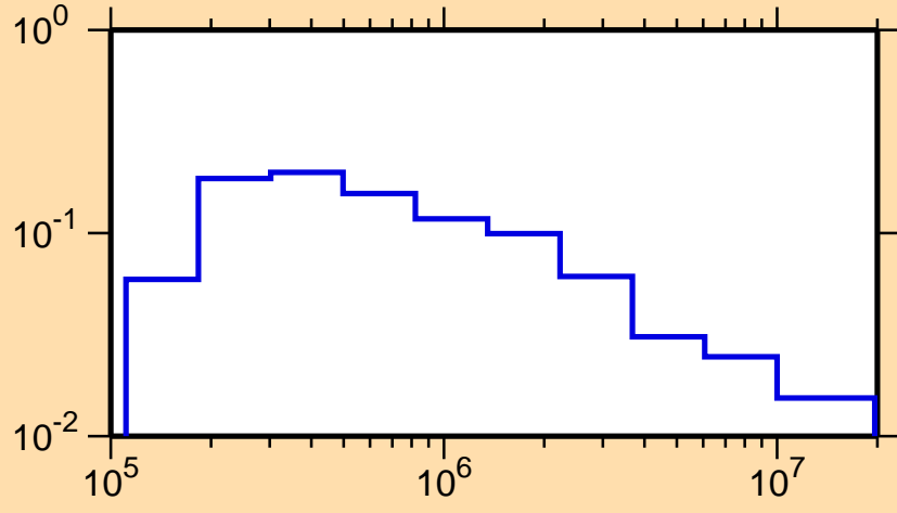
\sigma vs. E for ^{96}\text{Rh}(n,n_2)
