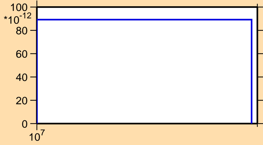
\sigma vs. E for ^{96}\text{Rh} (mt 34)
