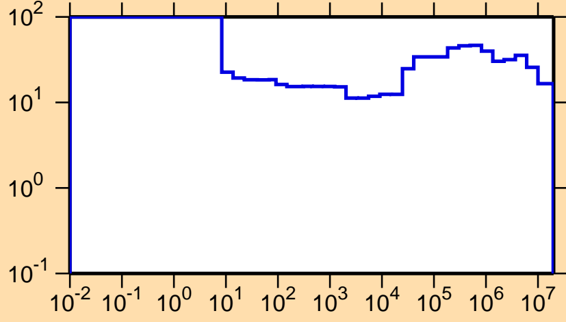
\Delta\sigma/\sigma vs. E for ^{96}\text{Rh}(n,p)
