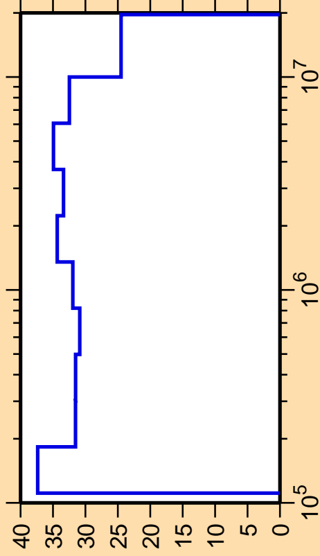
\Delta\sigma/\sigma vs. E for ^{96}\text{Rh}(n,n_4)
