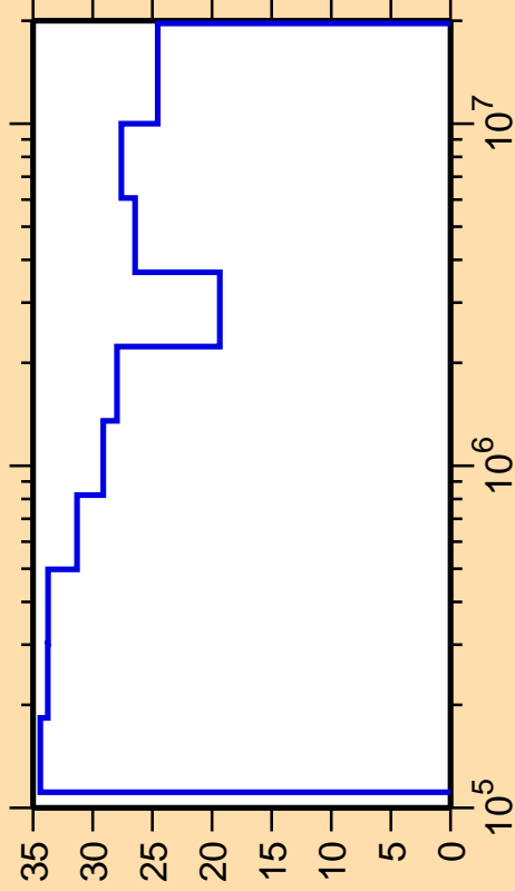
\Delta\sigma/\sigma vs. E for ^{96}\text{Rh}(n,n_2)
