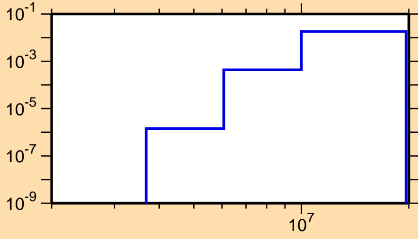
\sigma vs. E for ^{96}\text{Rh}(n,d)
