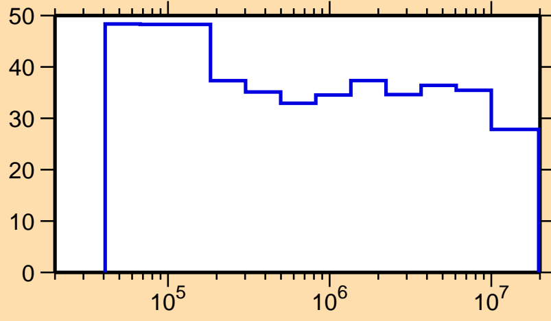
\Delta\sigma/\sigma vs. E for ^{96}\text{Rh}(n,n_1)
