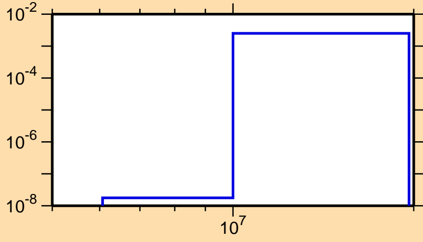
\sigma vs. E for ^{96}\text{Rh}(n,n\alpha)
