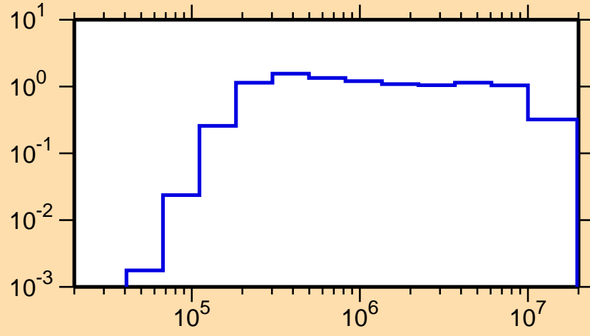
\sigma vs. E for ^{96}\text{Rh}(n,\text{inel.})
