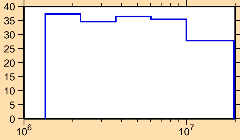
\Delta\sigma/\sigma vs. E for ^{96}\text{Rh}(n,n_1)
