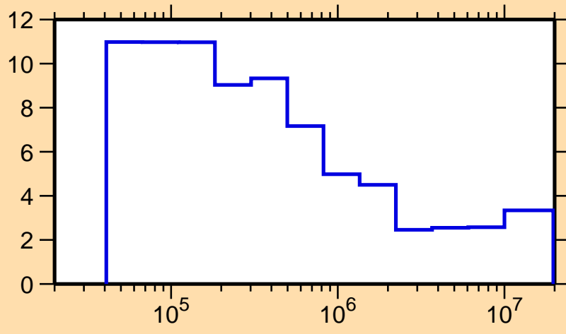
\Delta\sigma/\sigma vs. E for ^{96}\text{Rh}(n,\text{nonel.})
