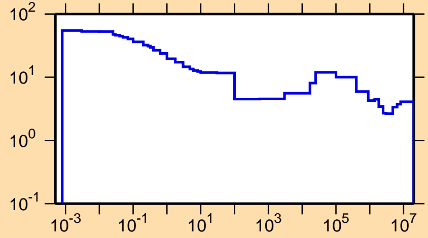
\Delta\sigma/\sigma vs. E for ^{96}\text{Rh}(n,\text{tot.})
