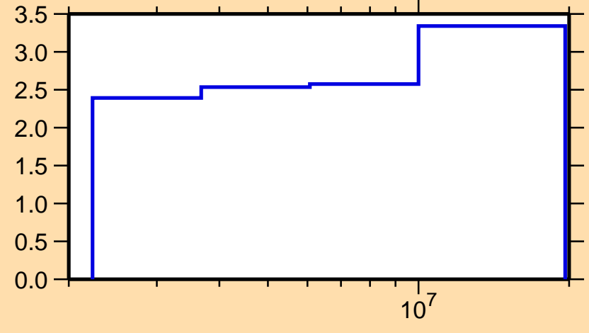
\Delta\sigma/\sigma vs. E for ^{96}\text{Rh}(n,n\text{nonel.})
