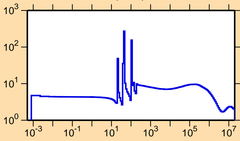
\sigma vs. E for ^{97}\text{Rh}(n,\text{el.})
