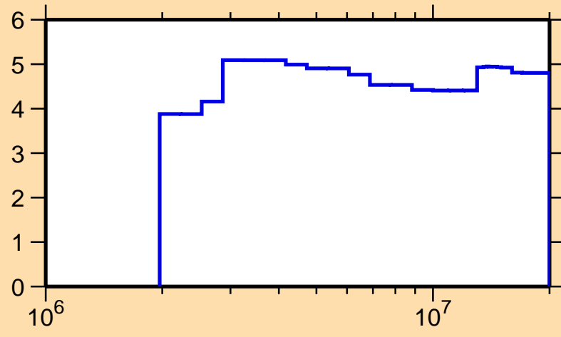
\Delta\sigma/\sigma vs. E for ^{97}\text{Rh}(n,n\text{onel.})
