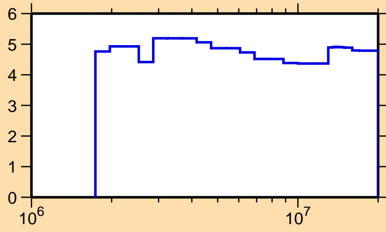
\Delta\sigma/\sigma vs. E for ^{97}\text{Rh}(n,n\text{nonel.})
