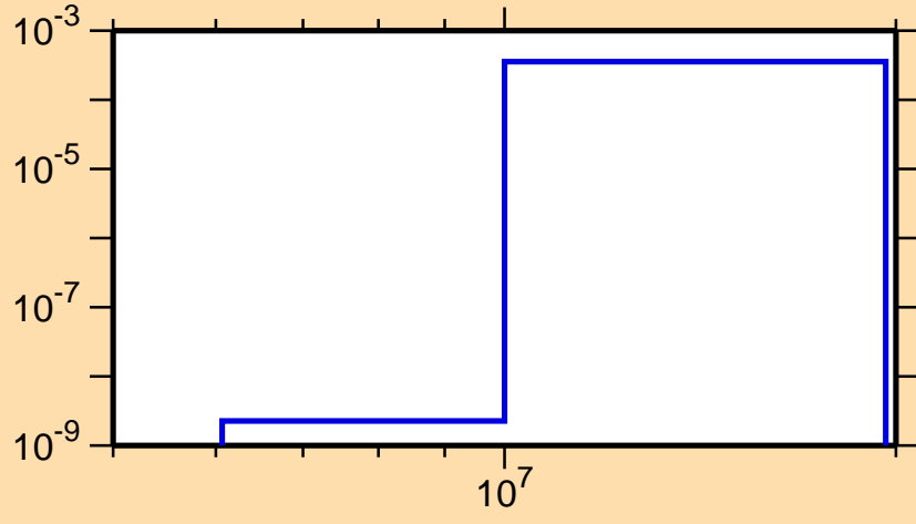
\sigma vs. E for ^{97}\text{Rh}(n,t)
