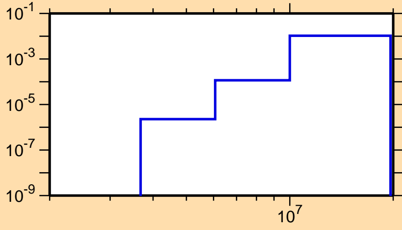
\sigma vs. E for ^{97}\text{Rh}(n,d)
