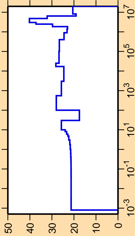
\Delta\sigma/\sigma vs. E for ^{97}\text{Rh}(n,\gamma)
