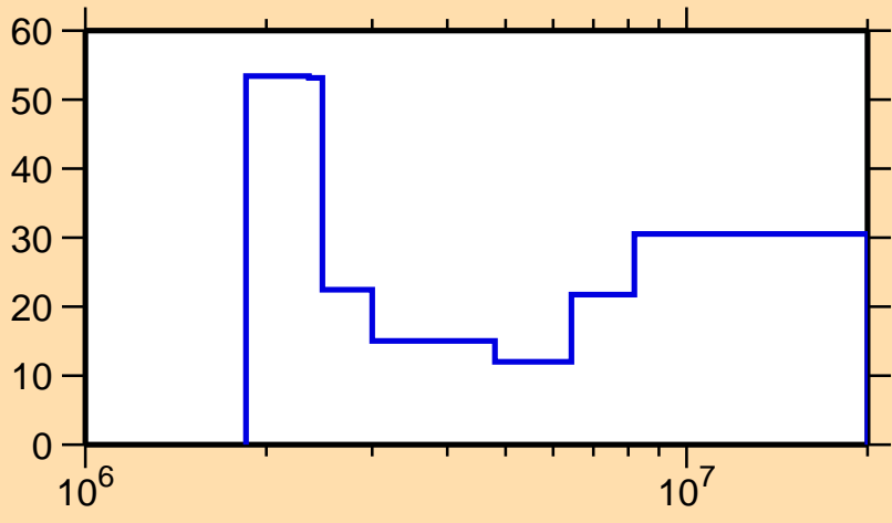
\Delta\sigma/\sigma vs. E for ^{97}\text{Rh}(n,ncont.)
