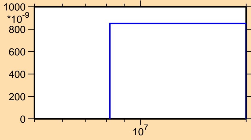
\sigma vs. E for ^{97}\text{Rh} (mt 45)
