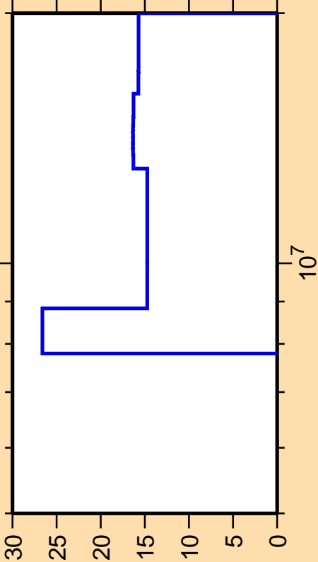
\Delta\sigma/\sigma vs. E for ^{98}\text{Rh}(n,2n)
