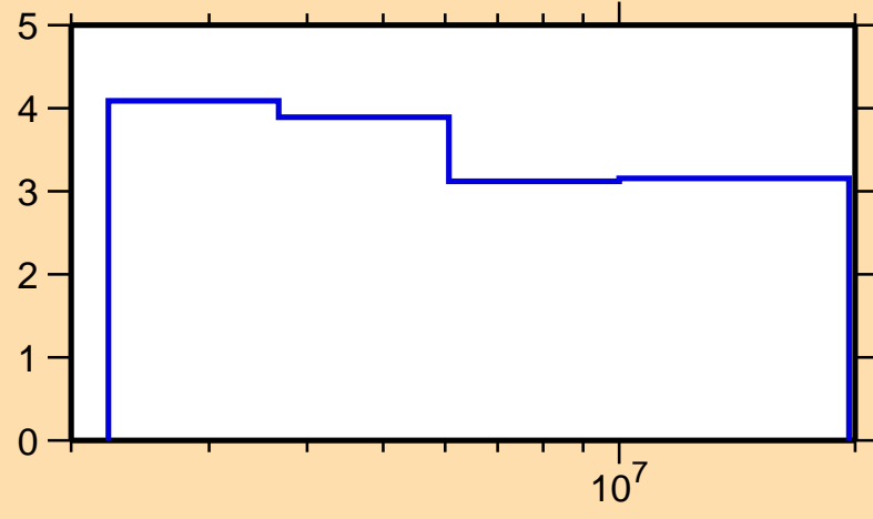
\Delta\sigma/\sigma vs. E for ^{98}\text{Rh}(n,n\text{onel.})
