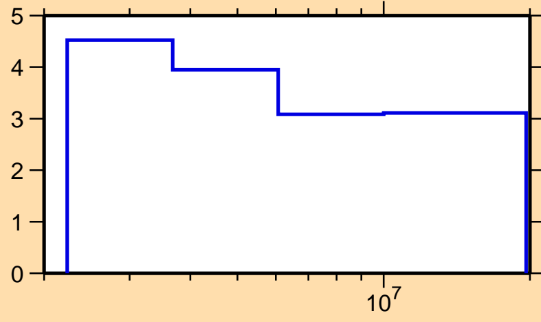
\Delta\sigma/\sigma vs. E for ^{98}\text{Rh}(n,n\text{nonel.})
