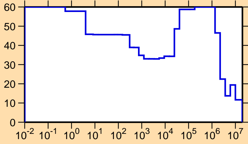
\Delta\sigma/\sigma vs. E for ^{98}\text{Rh}(n,p)
