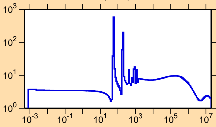
\sigma vs. E for ^{99}\text{Rh}(n,\text{el.})
