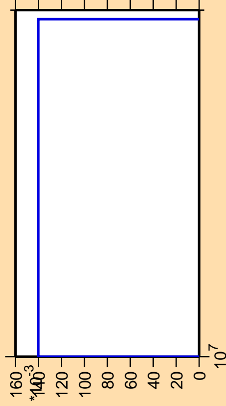
\Delta\sigma/\sigma vs. E for ^{100}\text{Rh} (mt 34)
