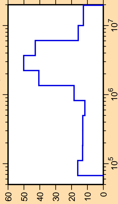
\Delta\sigma/\sigma vs. E for ^{100}\text{Rh}(n,n_3)
