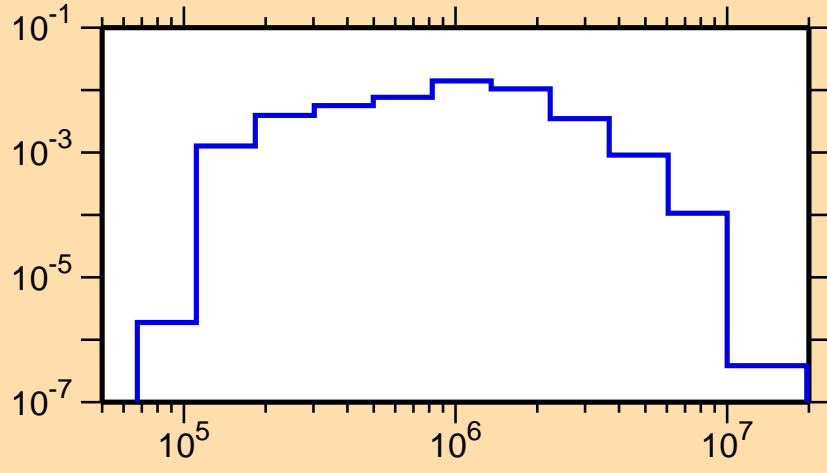
\sigma vs. E for ^{100}\text{Rh}(n,n_4)
