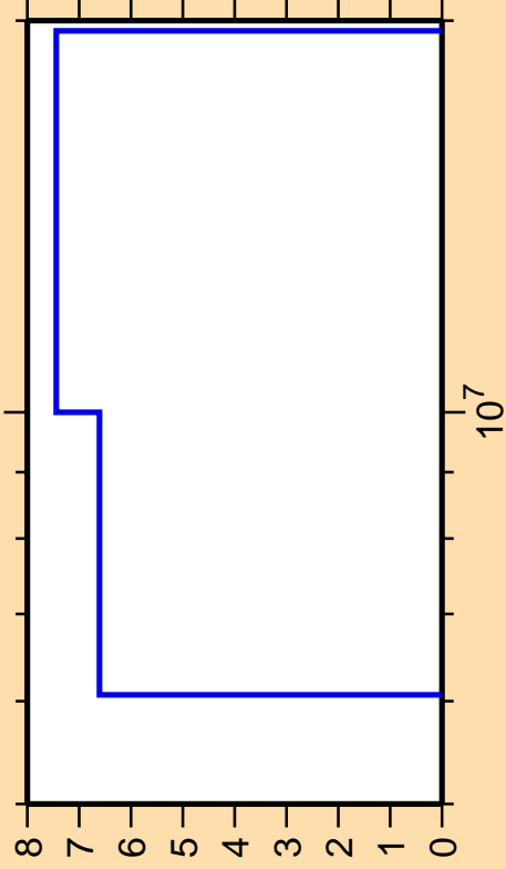
\Delta\sigma/\sigma vs. E for ^{100}\text{Rh}(n,2n)
