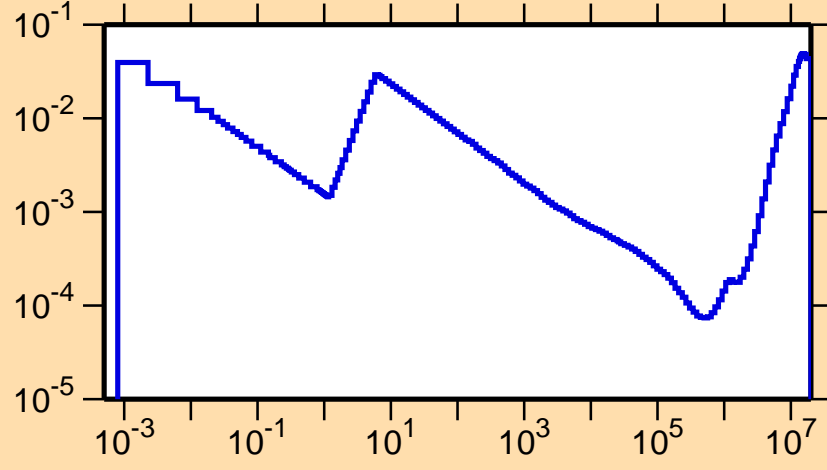
\sigma vs. E for ^{100}\text{Rh}(n,\alpha)
