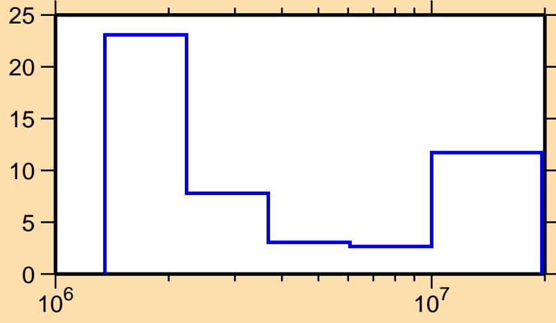
\Delta\sigma/\sigma vs. E for ^{101}\text{Rh}(n,n\text{cont.})
