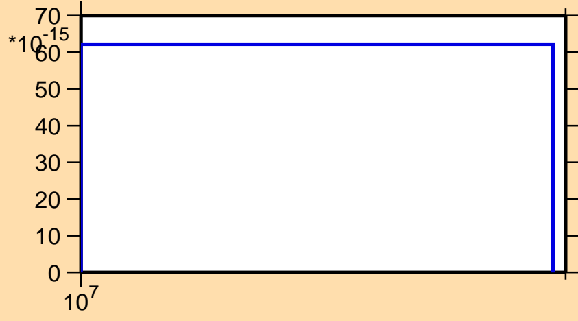
\sigma vs. E for ^{101}\text{Rh}(n,pd)
