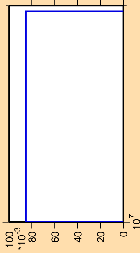
\Delta\sigma/\sigma vs. E for ^{101}\text{Rh}(n,pd)
