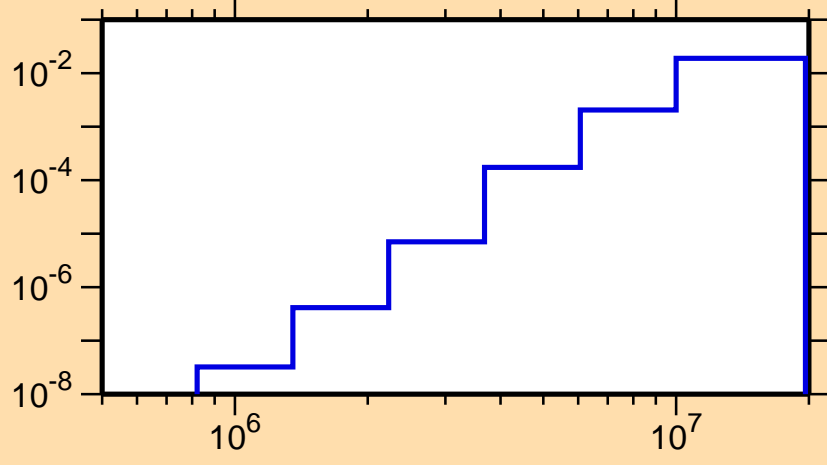
\sigma vs. E for ^{101}\text{Rh}(n,\alpha)
