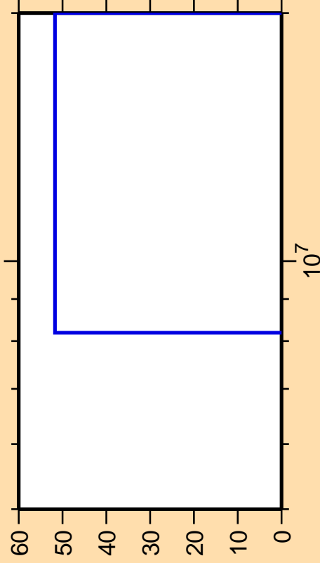
\Delta\sigma/\sigma vs. E for ^{101}\text{Rh}(n,nd)
