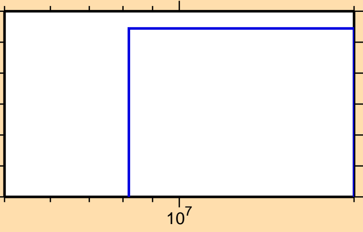
\sigma vs. E for ^{101}\text{Rh}(n,2np)
