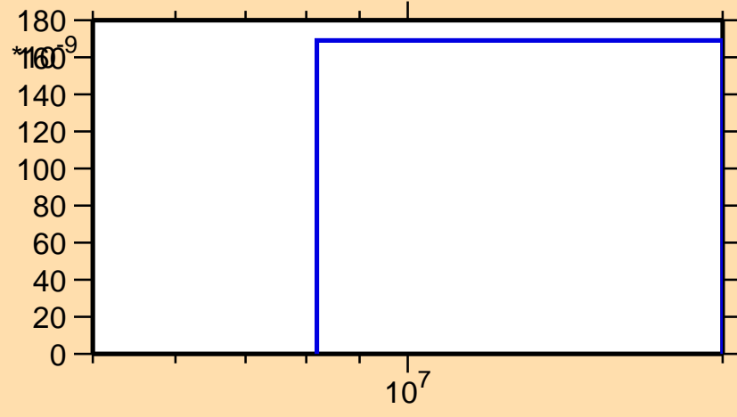
\sigma vs. E for ^{101}\text{Rh}(n,nd)
