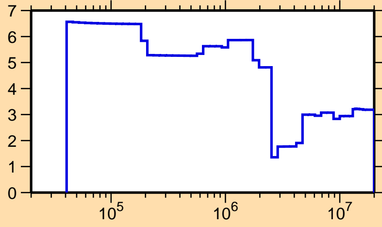
\Delta\sigma/\sigma vs. E for ^{102}\text{Rh}(n,\text{el.})
