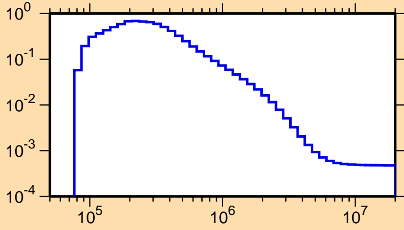
\sigma vs. E for ^{102}\text{Rh}(n,n_2)
