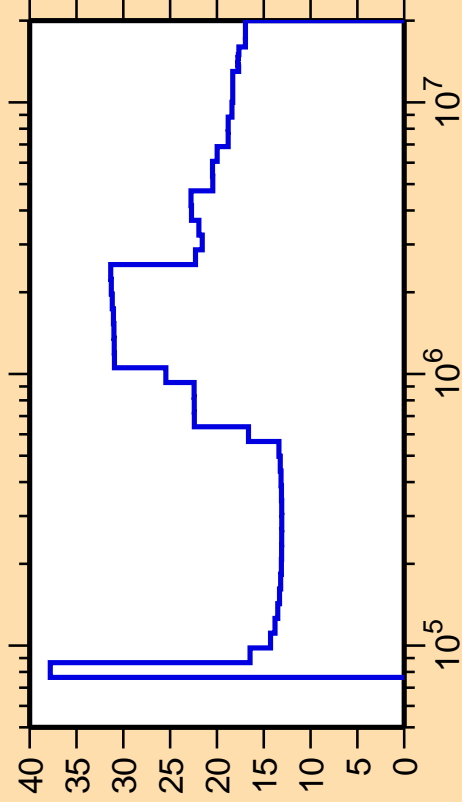
\Delta\sigma/\sigma vs. E for ^{102}\text{Rh}(n,n_2)
