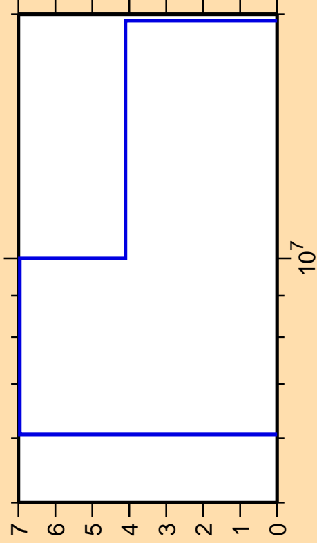
\Delta\sigma/\sigma vs. E for ^{102}\text{Rh}(n,2n)
