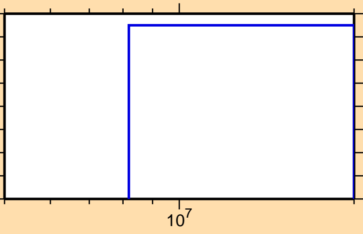
\sigma vs. E for ^{102}\text{Rh}(n,\text{He3})
