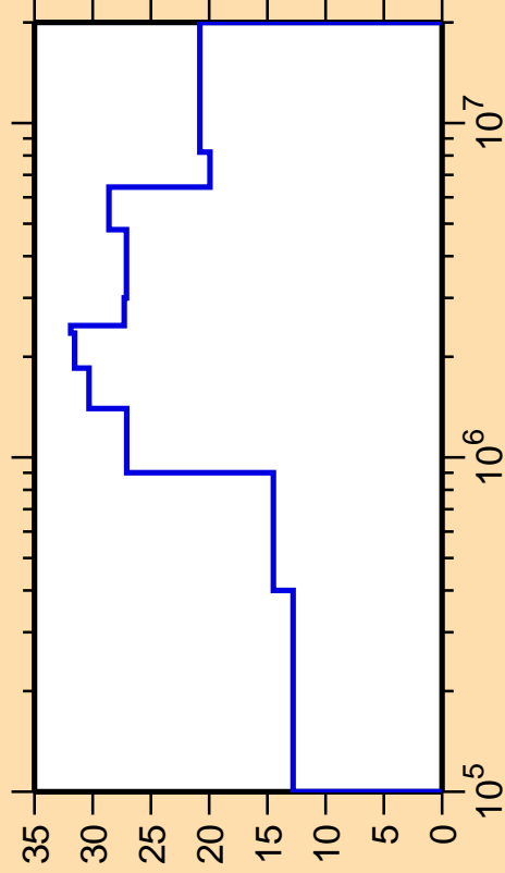
\Delta\sigma/\sigma vs. E for ^{102}\text{Rh}(n,n_4)
