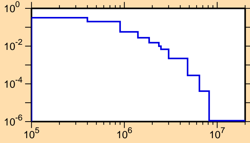
\sigma vs. E for ^{102}\text{Rh}(n,n_4)
