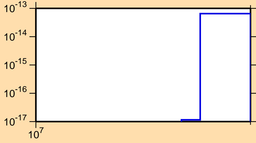
\sigma vs. E for ^{102}\text{Rh} (mt 34)
