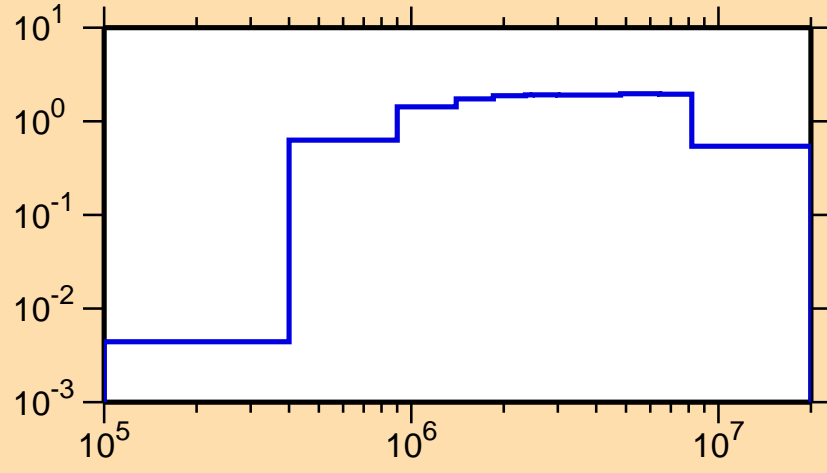
\sigma vs. E for ^{102}\text{Rh}(n,n\text{cont.})
