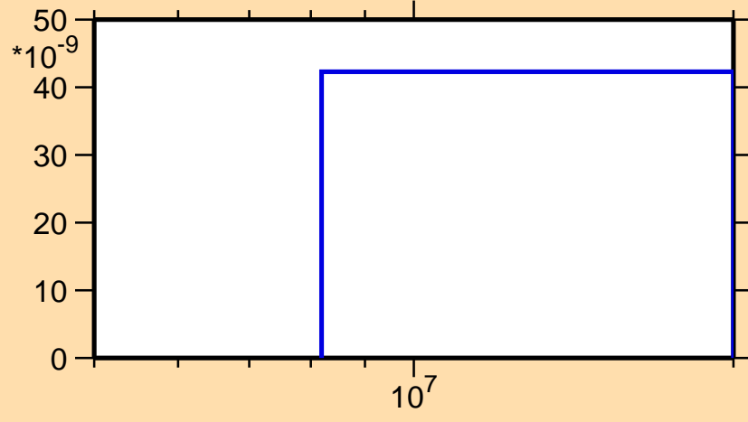
\sigma vs. E for ^{102}\text{Rh}(n,p\alpha)
