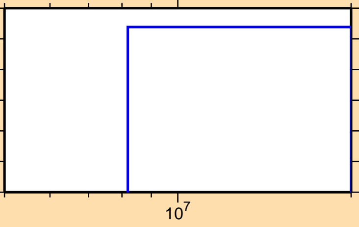
\sigma vs. E for ^{102}\text{Rh}(\text{mt117})
