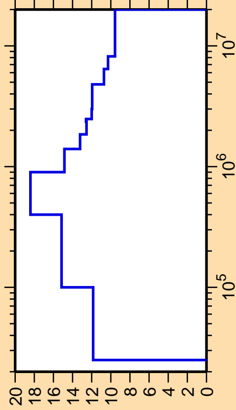
\Delta\sigma/\sigma vs. E for ^{103}\text{Rh}(n,n_1)
