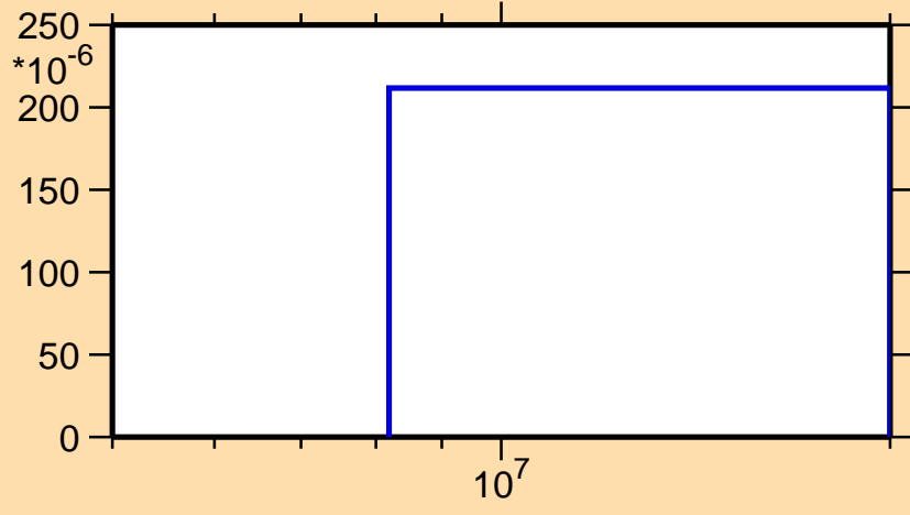
\sigma vs. E for ^{103}\text{Rh}(n,t)
