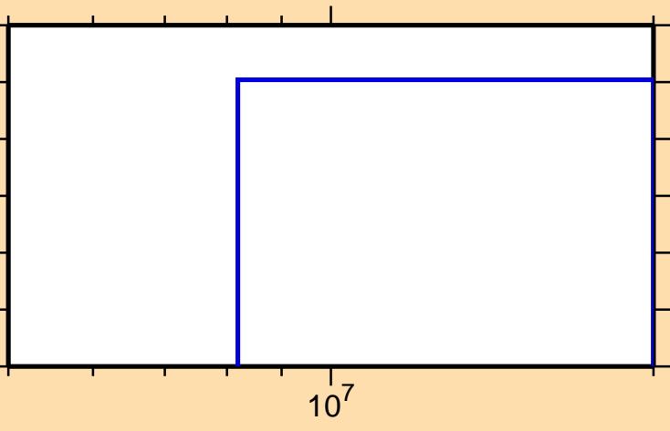
\sigma vs. E for ^{103}\text{Rh}(n,2np)
