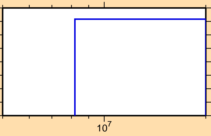
\sigma vs. E for ^{103}\text{Rh}(\text{mt117})
