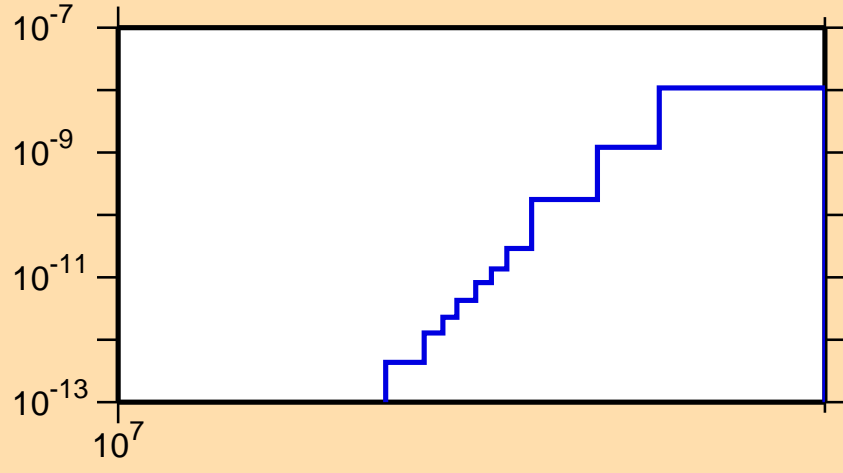
\sigma vs. E for ^{103}\text{Rh}(n,p\alpha)
