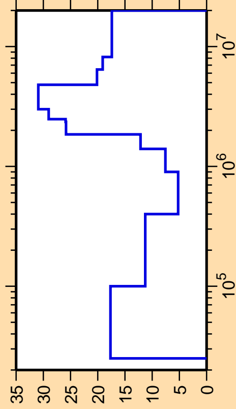
\Delta\sigma/\sigma vs. E for ^{103}\text{Rh}(n,n_2)
