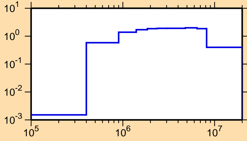
\sigma vs. E for ^{104}\text{Rh}(n,n\text{cont.})
