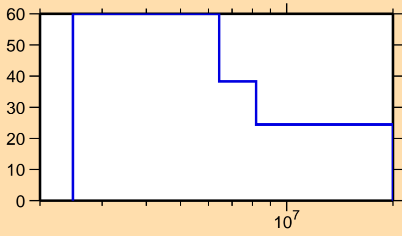
\Delta\sigma/\sigma vs. E for ^{105}\text{Rh}(n,p)
