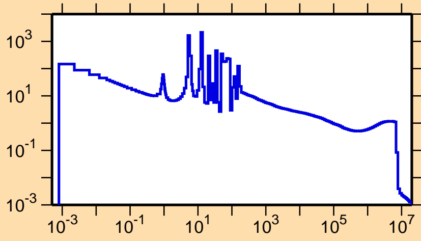
\sigma vs. E for ^{106}\text{Rh}(n,\gamma)
