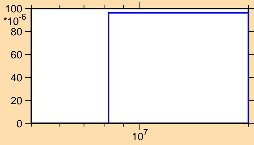
\sigma vs. E for ^{106}\text{Rh}(n,n\alpha)
