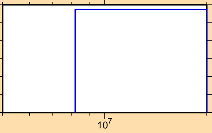
\sigma vs. E for ^{106}\text{Rh}(n,2n\alpha)
