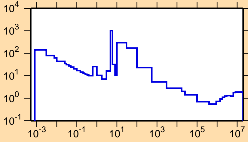
\sigma vs. E for ^{106}\text{Rh}(n,\text{nonel.})
