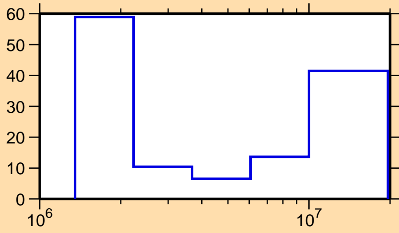
\Delta\sigma/\sigma vs. E for ^{106}\text{Rh}(n,n\text{cont.})
