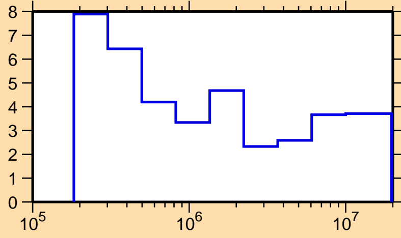
\Delta\sigma/\sigma vs. E for ^{107}\text{Rh}(n,\text{el.})
