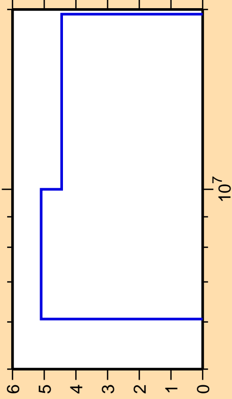
\Delta\sigma/\sigma vs. E for ^{107}\text{Rh}(n,2n)
