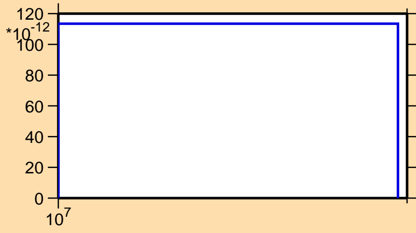
\sigma vs. E for ^{107}\text{Rh}(n,2np)
