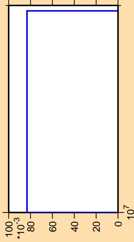
\Delta\sigma/\sigma vs. E for ^{107}\text{Rh}(n,2n\alpha)
