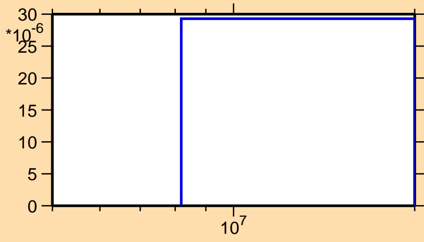
\sigma vs. E for ^{107}\text{Rh}(n,n\alpha)
