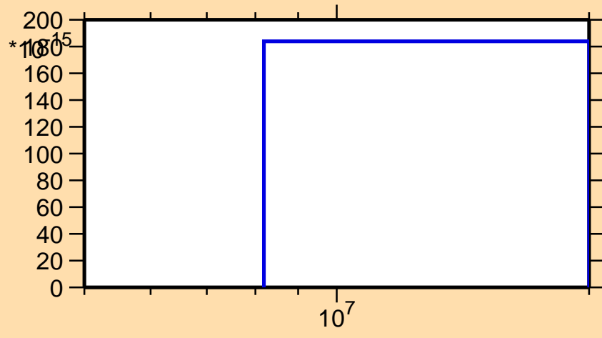
\sigma vs. E for ^{107}\text{Rh}(n,2n\alpha)
