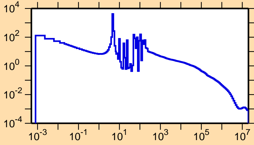
\sigma vs. E for ^{108}\text{Rh}(n,\gamma)
