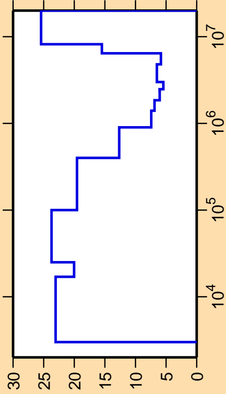
\Delta\sigma/\sigma vs. E for ^{108}\text{Rh}(n,\text{inel.})
