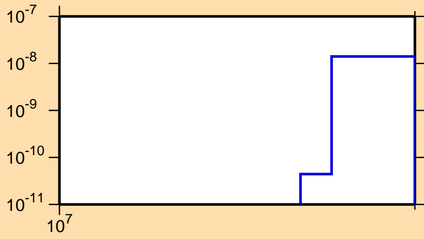
\sigma vs. E for ^{108}\text{Rh}(n,2n\alpha)
