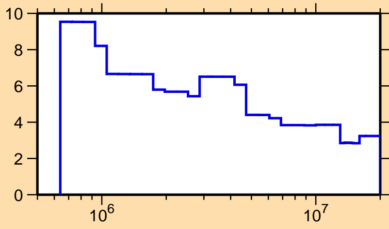
\Delta\sigma/\sigma vs. E for ^{108}\text{Rh}(n,n\text{nonel.})
